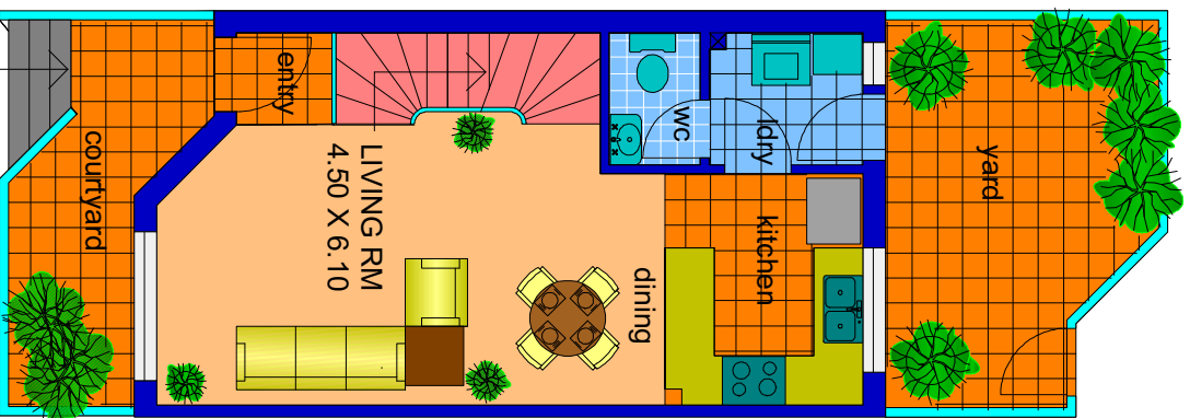
LOWER LEVEL
